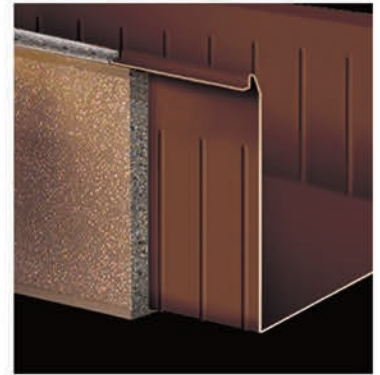
Fiberlon® or Durapreme® Liner Bonded to Decorative Finish 5000 PSI Reinforced Concrete
